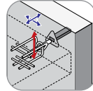
Egcodorn® SWQ for longitudinal and transverse movement
