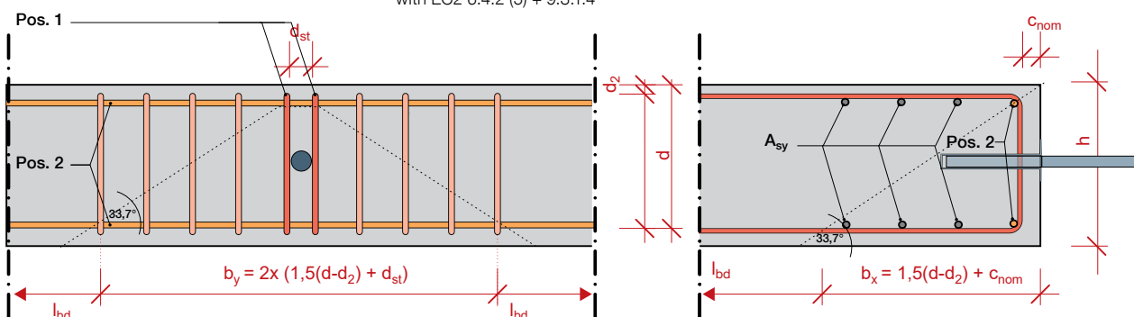
Pos. 1 or edge reinforcement in accordance with EC2 6.4.2 (5) + 9.3.1.4
